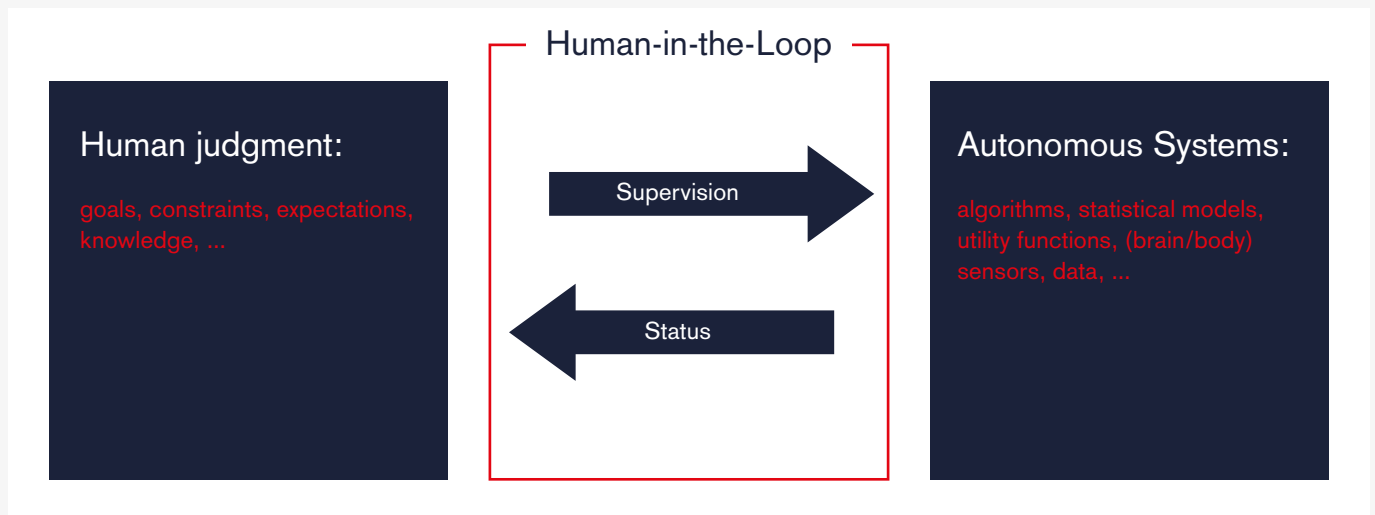
Figure 3.1. Human-in-the-loop (Rahwan, 2016)
