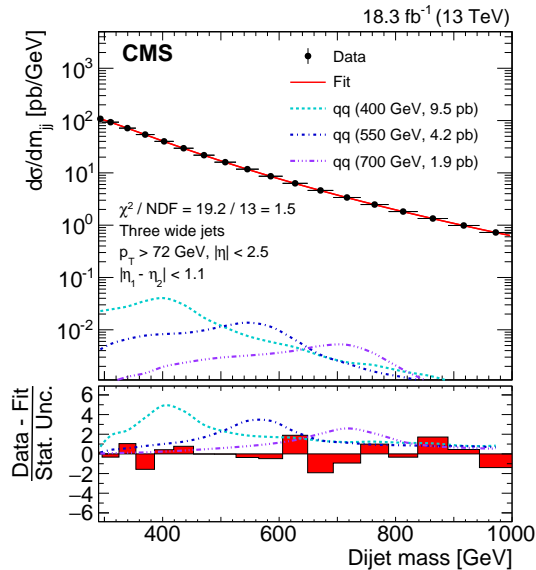
Figure 1: Dijet mass spectrum (points) compared to a fitted parameterization of the background (solid curve), where the fit is performed in the range 290 < m_{jj} < 1000 GeV. The horizontal bars show the widths of each bin in dijet mass. The dashed lines represent the dijet mass distribution from 400, 550, and 700 GeV resonance signals expected to be excluded at 95% CL by this analysis. The lower panel shows the difference between the data and the fitted parametrization, divided by the statistical uncertainty of the data.
