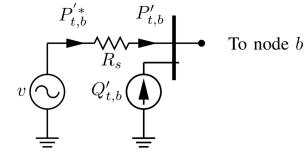
Fig. 2. Equivalent circuit model of the battery energy storage system. P'_{t,b}, Q'_{t,b} are the active and reactive power injections of the battery. P'_{t,b} is the 'lossy' active power injection that is used to drive the model of state-of-energy of the battery.
