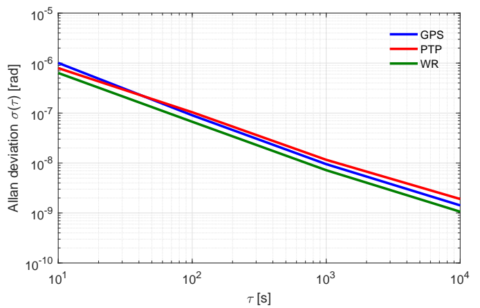
Fig. 11. Worst-case scenario: phase error Allan deviation over a 24-hour test, for GPS (blue), PTP (red) and WR (green) PMUs. The test waveform consists of a single fundamental tone whose amplitude, frequency and phase are set equal to 300 V, 50 Hz, and 0 rad, respectively.
