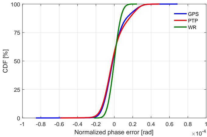
Fig. 5. Phase error cumulative distribution functions as provided by GPS (blue), PTP (red) and WR (green) PMUs over a test duration of 24 hours. The test waveform consists of a single fundamental tone whose amplitude, frequency and phase are set equal to 300 V, 47.5 Hz, and 0 rad, respectively.
