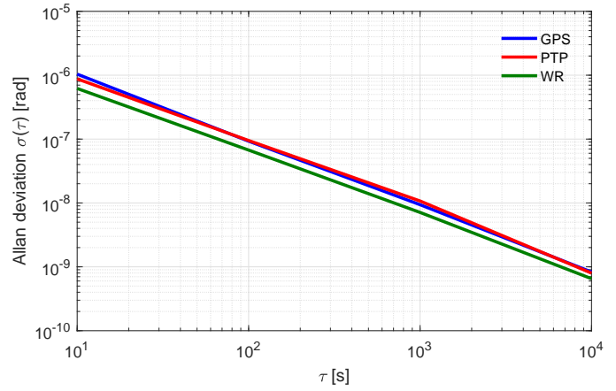
Fig. 8. Phase error Allan deviation as function of the time interval \tau , for GPS (blue), PTP (red) and WR (green) PMUs over a test duration of 24 hours. The test waveform consists of a single fundamental tone whose amplitude, frequency and phase are set equal to 300 V, 47.5 Hz, and 0 rad, respectively.
