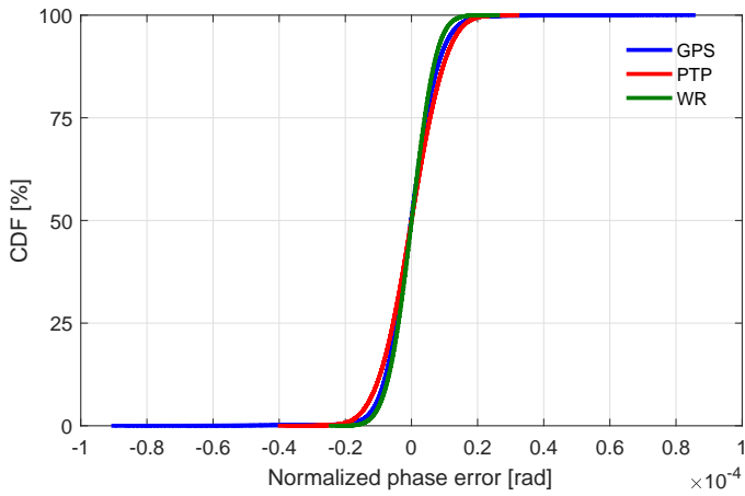
Fig. 4. Phase error cumulative distribution functions as provided by GPS (blue), PTP (red) and WR (green) PMUs over a test duration of 24 hours. The test waveform consists of a single fundamental tone whose amplitude, frequency and phase are set equal to 300 V, 50 Hz, and 0 rad, respectively.
