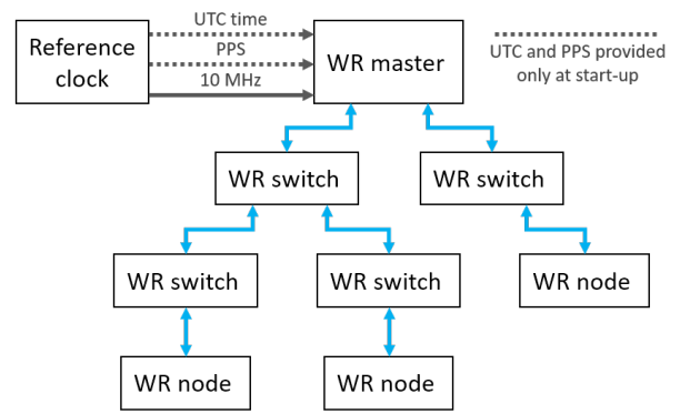
Fig. 1. White Rabbit network architecture.
