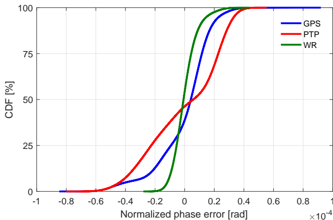
Fig. 10. Worst-case scenario: phase error cumulative distribution function over a 24-hour test, for GPS (blue), PTP (red) and WR (green) PMUs. The test waveform consists of a single fundamental tone whose amplitude, frequency and phase are set equal to 300 V, 50 Hz, and 0 rad, respectively.
