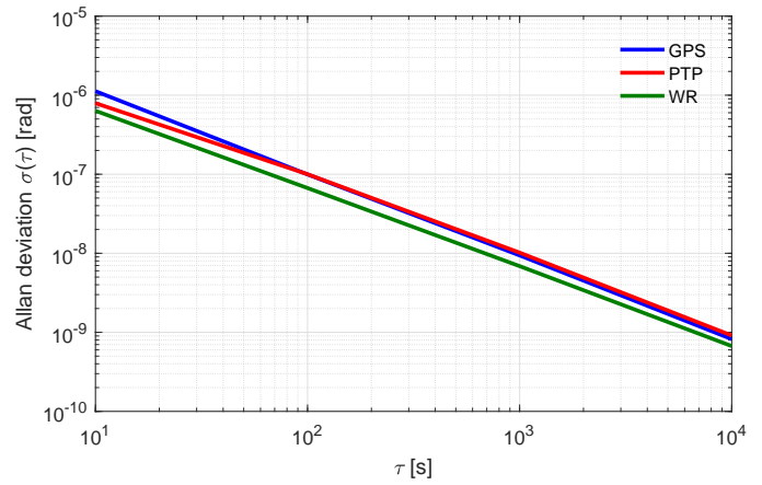
Fig. 7. Phase error Allan deviation as function of the time interval \tau , for GPS (blue), PTP (red) and WR (green) PMUs over a test duration of 24 hours. The test waveform consists of a single fundamental tone whose amplitude, frequency and phase are set equal to 300 V, 50 Hz, and 0 rad, respectively.
