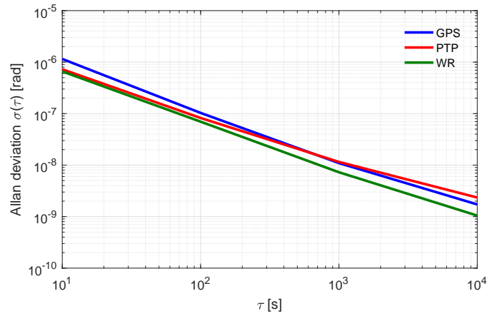
Fig. 9. Phase error Allan deviation as function of the time interval \tau , for GPS (blue), PTP (red) and WR (green) PMUs over a test duration of 24 hours. The test waveform consists of a single fundamental tone whose amplitude, frequency and phase are set equal to 300 V, 52.5 Hz, and 0 rad, respectively.
