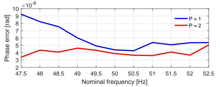
Fig. 2. Phase estimation error as provided by e-IPDFT as function of the fundamental frequency, when the iteration number P of the compensation routine is set equal to 1 (blue) and 2 (red), respectively. The additive white Gaussian noise produces a signal-to-noise ratio of 85 dB.
