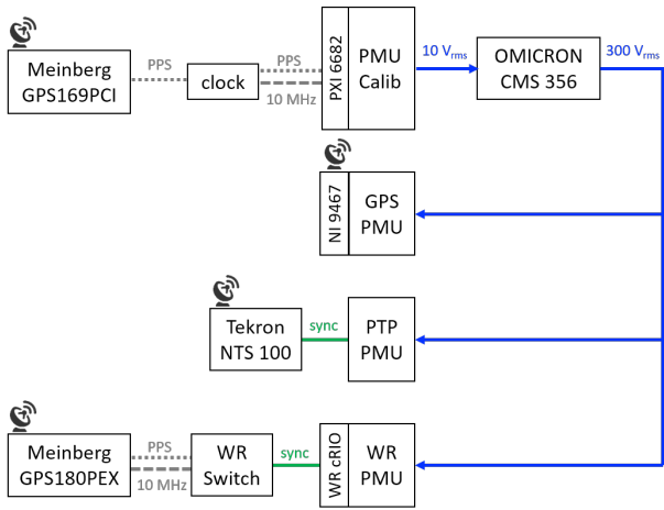
Fig. 3. Measurement setup for the assessment of the PMUs' phase estimation accuracy. The PMU calibrator generates the user-defined test waveforms, that are amplified up to 300 V by the CMS 356 OMICRON amplifier, and then supplied to the three considered PMUs, relying on GPS, PTP and WR time dissemination, respectively.
