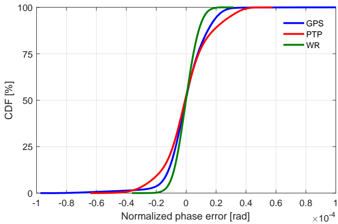
Fig. 6. Phase error cumulative distribution functions as provided by GPS (blue), PTP (red) and WR (green) PMUs over a test duration of 24 hours. The test waveform consists of a single fundamental tone whose amplitude, frequency and phase are set equal to 300 V, 52.5 Hz, and 0 rad, respectively.
