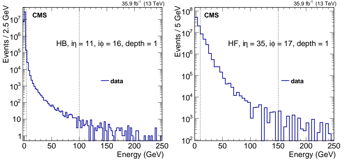
Figure 2: Energy spectra used as an input to the iterative method of equalizing the \phi response of one typical i\eta ring for an HB (left) and HF (right) calorimeter channel. Energy thresholds on the deposits used for the energy estimation are shown with dashed lines. The legends show the HCAL channel index in i\eta , i\phi , and depth segmentation units.
