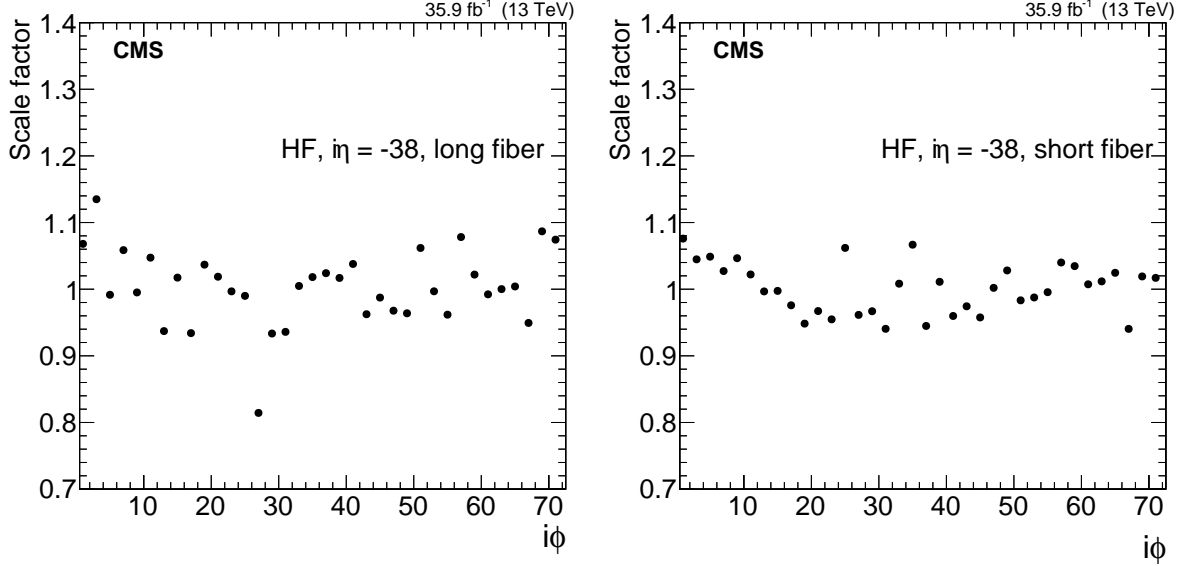
Figure 4: Calibration scale factor obtained using the method of moments with the first moment of the energy distribution for long (left) and short (right) fibers for two typical HF channels with i\eta = -38 , as a function of i\phi . Only statistical uncertainties in the measurements are shown in these plots.
