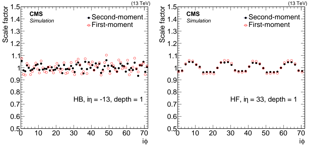
Figure 5: Derived calibration scale factors that equalize the \phi response in a simulated sample of minimum bias events for a channel in the HB ( i\eta = -13 , depth = 1, left) and HF ( i\eta = 33 , depth = 1, right), as a function of i\phi using two different methods: of first and of second moment.
