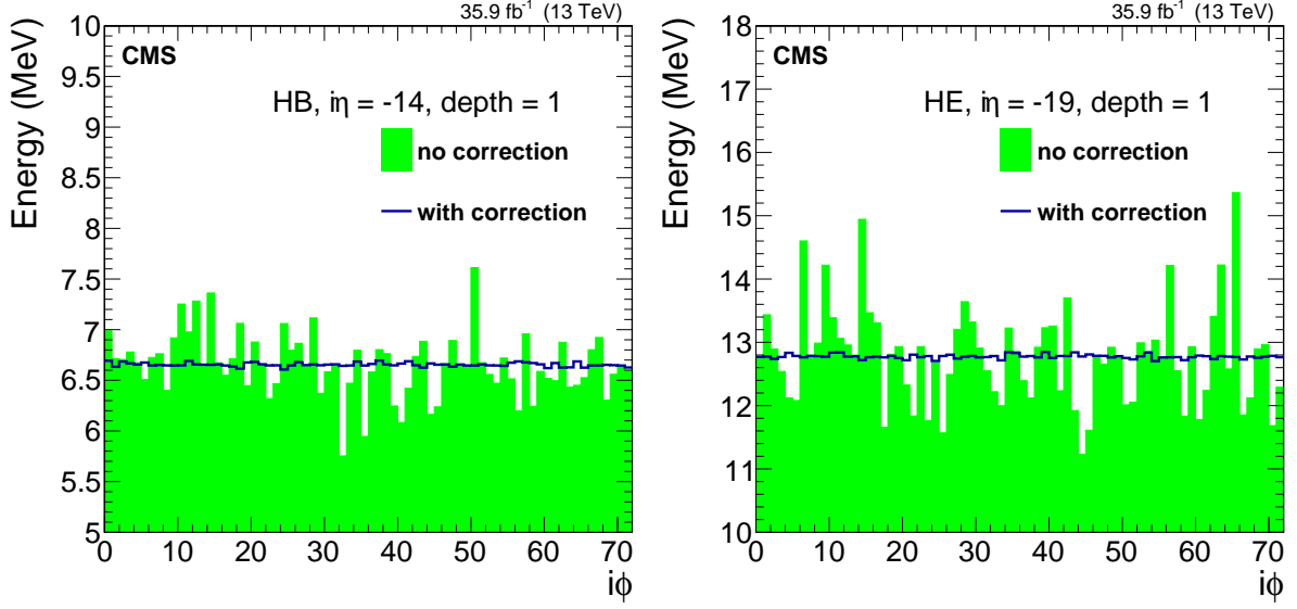
Figure 3: Mean cell energy \langle E_{\text{tot}} \rangle for the iterative method measured before (solid histogram) and after (open histogram) correction as a function of i\phi for a typical i\eta ring of the HB ( i\eta = -14 , depth = 1, left) and of the HE ( i\eta = -19 , depth = 1, right) calorimeters. Data triggered using electrons, photons, and muon are used in this calibration procedure.
