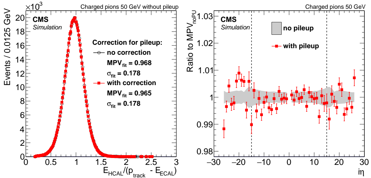
Figure 8: left: Distribution of the energy response in a simulated sample of single isolated high- p_T pions without pileup when the corrections for pileup have (red squares) or have not (black circles) been applied. The plot also shows the results of Gaussian fits. right: The ratio of the mode of the response distribution for a simulated pion sample with pileup, with loose charged-particle isolation, and the correction for pileup applied (red squares) to the mode from the sample without pileup. The uncertainties in the mode without pileup are shown with the gray band. Only statistical uncertainties are included. The dashed vertical lines show the boundaries between the barrel and the endcaps.
