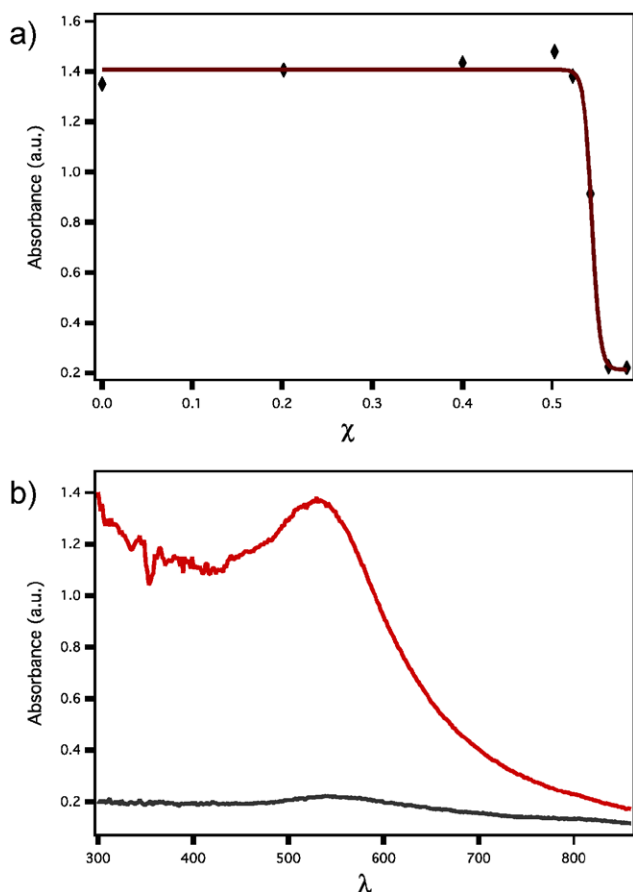
Figure 1. Example of a titration experiment—MUA-OT 4 : 1 nanoparticles titrated with TMA nanoparticles. (a) Absorbance at surface plasmon resonance maximum at different charge ratios, \chi . Experimental data (solid diamond) is fitted with sigmoid function (solid line). (b) UV-vis absorbance curves before (red, upper line) and after (black, lower line) the precipitation point.
