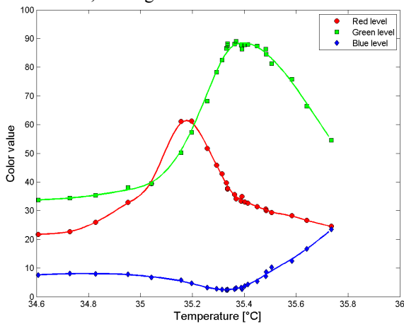
Figure 4: RGB values of the liquid crystals as a function of the temperature. Solid lines are spline fittings of the data.
