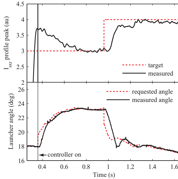
Figure 5. Real time peak-in-profile control for pulse 35857. The soft x-ray profile is fit with a spline in real time and the peak is compared to the target. At the step increase, the controller requested a smaller angle such that the ECRH deposition becomes more centralised and the soft x-ray emission increases.
