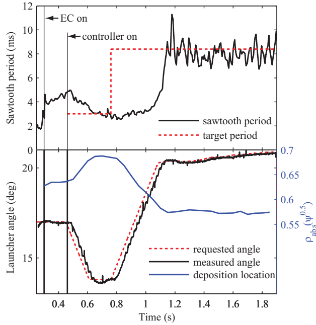
Figure 4. Real time, closed loop control of the sawtooth period for shot 35833. The target sawtooth period reference signal was initially 3ms, with a step to 8.5ms at 0.75s. The controller moves the launcher to successfully obtain and track the target. Also shown is the post shot calculation of the deposition in rho of the EC beam.
