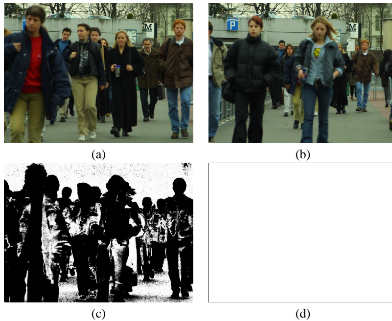
Figure 6: Illustration of the outlier mixture model. The images in Figure (a) and (b) are compared. For each pixel, the probability that it belongs to the outliers is shown by its greyscale value: in (c) using our outlier model and in (d) using a uniform distribution to model the outliers. (d) shows a total failure of the uniform model—the system tagged everything as inlier with a large variance. This shows that by using our model we can substantially improve the outlier resilience at the lowest level of a computer vision algorithm.
