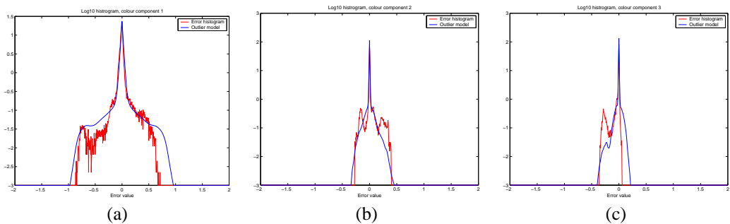
Figure 5: Comparison between the outlier mixture model and the error histogram of the images in Figure 3. The logarithm (in base 10) of the error histogram is plotted against the mixture model. (a) First colour component \alpha —the one with the largest singular value. (b) second colour component \beta (c) third colour component \gamma .
