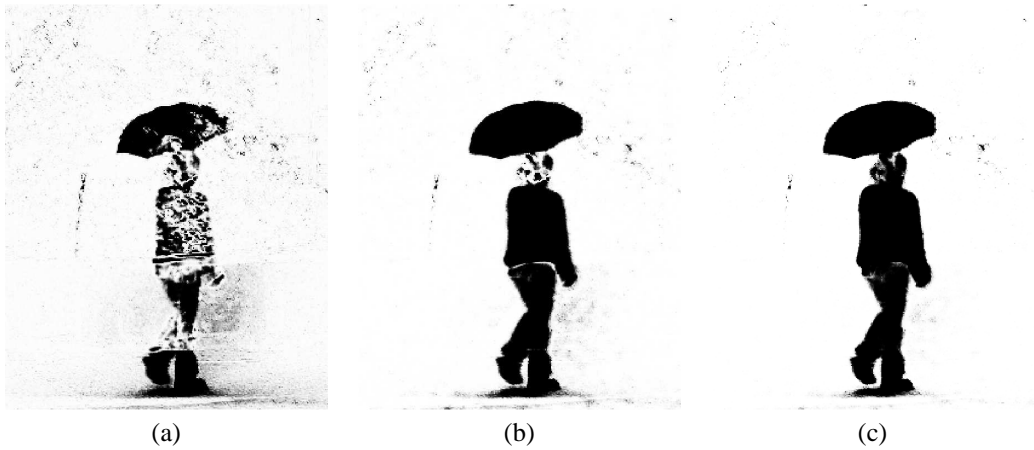
Figure 4: Illustration of the outlier mixture model. The images in Figure 3 are compared. For each pixel, the probability that it belongs to the outliers is shown by its greyscale value. (a) is using only the first colour channel (b) uses the first two colour channels (c) uses all the colour information to compute the model parameters.
