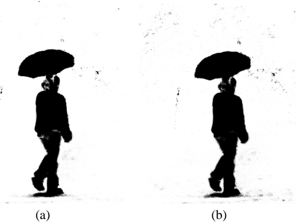
Figure 8: Comparison between the separable and non separable outlier model. (a) outlier mask obtained using 3 separate colour components (Same as Figure 5c). (b) outlier mask using the 3D outlier model of Equation (5). The three-dimensional model is slightly better at separating the outliers from the background, but its computation cost is prohibitive.
