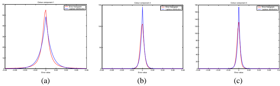
Figure 2: Error distribution computed on two consecutive images of the same scene, shown for the three colour channels. (a) \alpha channel. (b) \beta channel. (c) \gamma channel. Because of acquisition noise, and because of a slight displacement of the camera between the two views (less than one pixel in amplitude), the images are not exactly alike. The histogram of the error is compared to a laplacian distribution, showing that the laplacian is appropriate to model the inliers.
