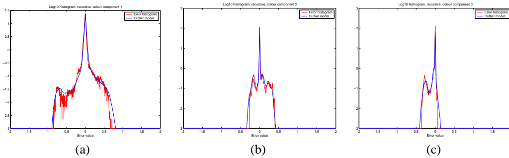
Figure 7: Same as Figure 5 but computing a second iteration of the outlier modelling. We can see that the model better predicts the error histogram.
