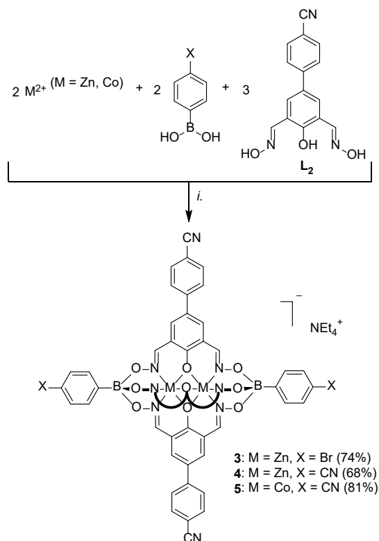
Scheme 3 Synthesis of the tri- and pentatopic clathrochelate complexes 3–5 . Reagents and conditions: (i): 4-bromo- or 4-cyanophenylboronic acid, dioxime ligand L2 , Zn(OTf) 2 or [Co(H 2 O) 6 ](NO 3 ) 2 , MeOH/EtOH, 70 °C, then NEt 4 OH.
