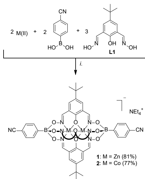
Scheme 1 Synthesis of the ditopic clathrochelate complexes 1 and 2 . Reagents and conditions: (i): [Co(H 2 O) 6 ](NO 3 ) 2 or Zn(OTf) 2 , EtOH/MeOH, 70 °C, then NEt 4 OH.
