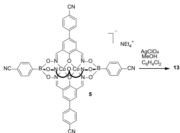
Scheme 8 Synthesis of coordination polymer 13 using pentatopic clathrochelate 5 .
