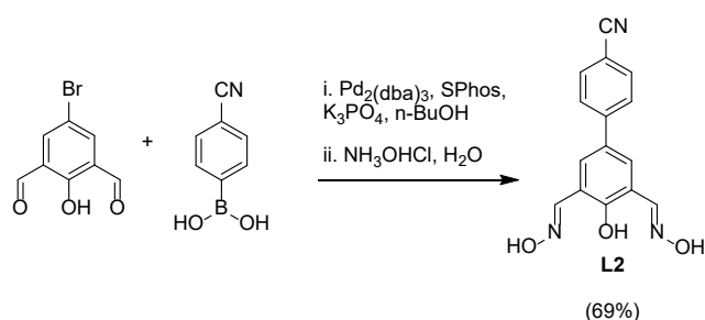
Scheme 2 Synthesis of the dioxime ligand L2 .
