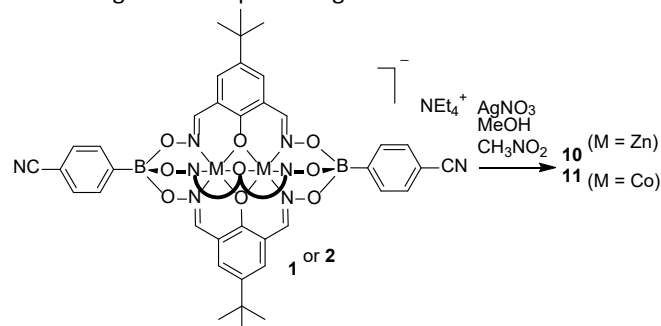
Scheme 6 Synthesis of the heterometallic coordination polymers 10 and 11 .
