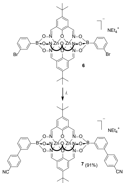
Scheme 4 Synthesis of the extended ditopic clathrochelate complex 7 . Reagents and conditions: (i.): 6 (1 eq.), 4-cyanophenylboronic acid (8 eq.), K_3PO_4 (4 eq.), Pd_2(dba)_3 (5 mol%), SPhos (10 mol%), n -BuOH/toluene (1:1), 90 °C, 14 h.
