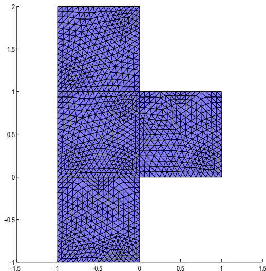
Figure 1: Mesh for the reduced-basis problem (normalized domain ).
