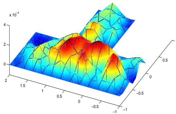
Figure 7: Distributed error \tilde{e} over the domain \Omega between \tilde{u} and u_N .
