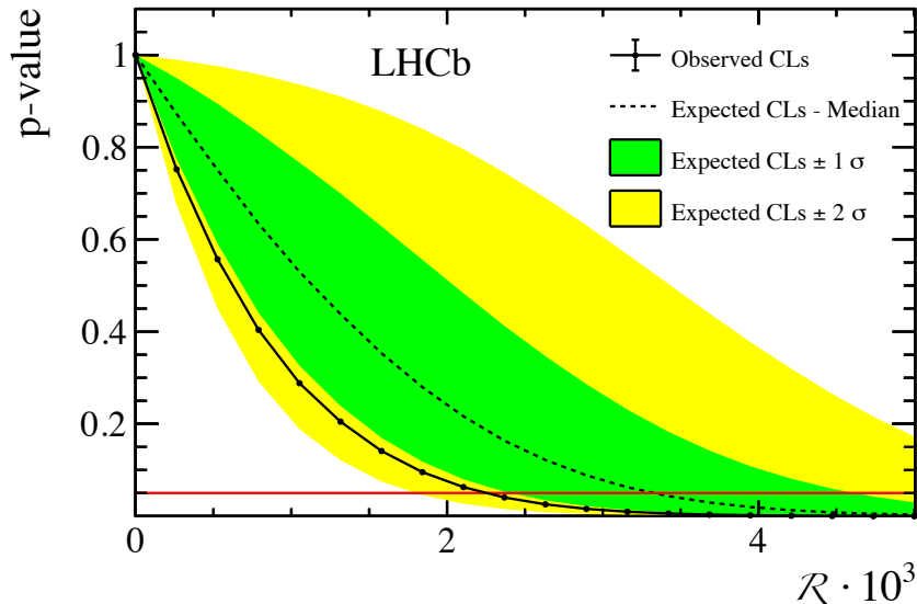
Figure 3: Result of the hypothesis tests conducted using the CLs method by varying \mathcal{R} is shown. The observed CLs distribution is shown by the round (black) points. The expected CLs distribution (based on the background only hypothesis) is shown by the dashed line (black), with 1 and 2 \sigma uncertainty bands depicted in dark shaded (green) and light shaded (yellow) bands. The observed and expected upper limits are obtained by seeing where the bands cross the p-value of 0.05 shown as the horizontal (red) line.
