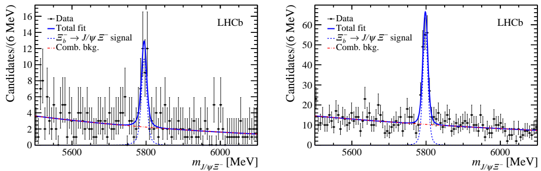
Figure 5: Distributions of J/\psi\xi^- mass shown as points with error bars for (left) Run 1 and (right) Run 1 data. The total fit to data is shown as a solid (blue) curve. The \xi_b^- \rightarrow J/\psi\xi^- signal is fit with the sum of two Crystal Ball functions with the same mean and width, but different tail parameters, shown as the dashed (blue) curve. The combinatorial background shape is fit with an exponential function, shown as a dashed (red) curve.
