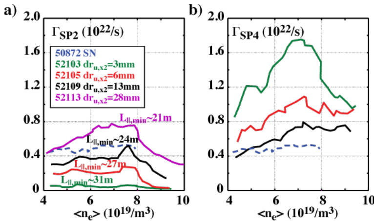
FIG. 6. Ion currents to (a) SP2 (lower primary inner-wall strike point) and (b) SP4 (outermost secondary strike point) for density ramps in LFS SF- configurations for varying X-point separation dr_{u,x2} . (Reproduced from [16].)
