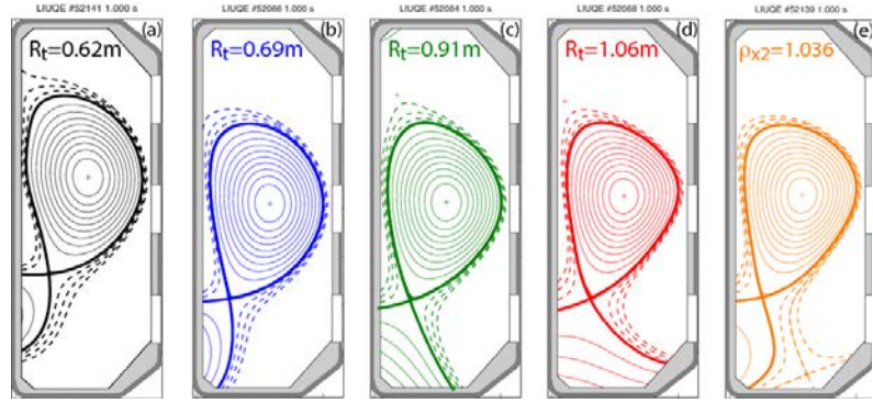
FIG. 4. Flux-surface contours of TCV equilibria for (a-d) varying major radius of the outer strike point, up to the super-X case, (e) X-point-target divertor. (Adapted from [17].)
