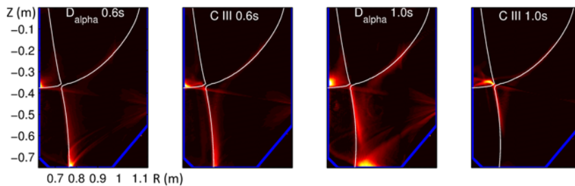
FIG. 5. D_\alpha and C III emissivity profiles 0.4 s before and at the onset of detachment (occurring at 1.0 s). (Reproduced with permission from [22].)
