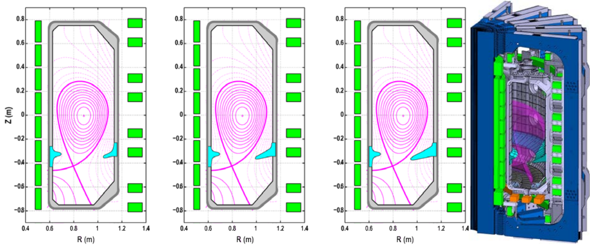
FIG. 11. (Left) Sketches of baffles for varying divertor closure, limiting the SOL at the flux surface with an outboard midplane separatrix separation of \sim 1 cm, 2 cm, and 3 cm, respectively, with centered X-point. (Right) 3D view for the case with the longest baffles. (Reproduced from [4].)
