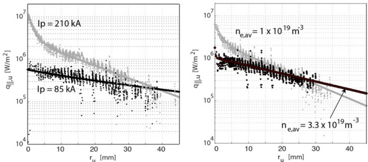
FIG. 7. Profiles of parallel heat flux to the target mapped to the outboard midplane in inboard limited plasmas for (left) two current values at line-averaged density 1.7 \times 10^{19} \text{ m}^{-3} and (right) two density values at a plasma current of 140 kA. (Reproduced from [28].)
