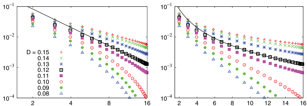
FIG. 6. (Color online) The amplitude of transverse spin correlations (15) as a function of the chord distance (16) on a log-log plot (left-hand side) and a simple log plot (right-hand side).
