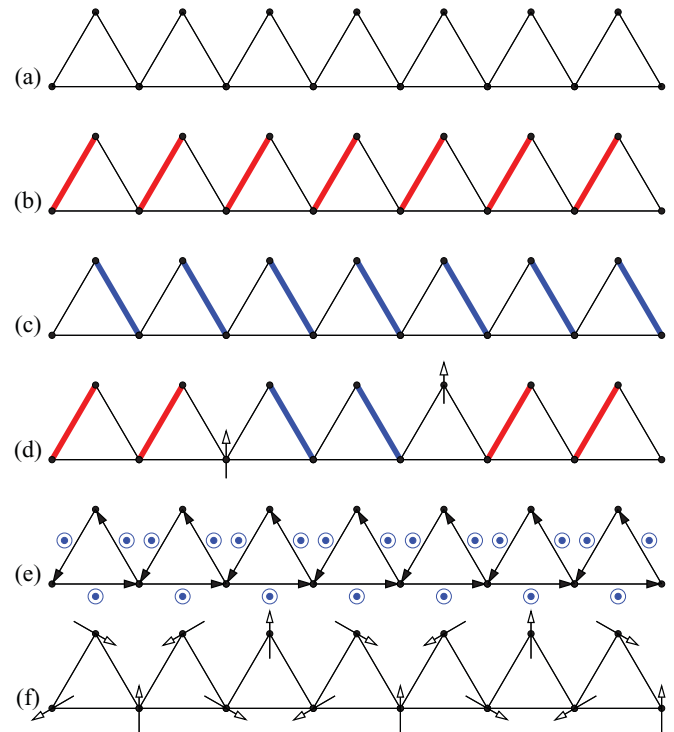
FIG. 2. (Color online) (a) The sawtooth chain. (b) and (c) Its valence-bond ground states. (d) Spin-1/2 excitations: kink (left-hand side) and antikink (right-hand side). (e) Orientation of the DM vectors \mathbf{D}_{ij} . (f) The ground state of the classical model has a commensurate magnetic order with the wave number q/2\pi = -1/3 .
