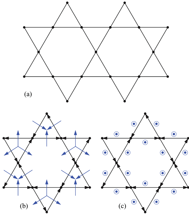
FIG. 1. (Color online) (a) Kagome lattice. (b) and (c) In-plane and out-of-plane components of the DM vector \mathbf{D}_{ij} shown for directed links ( i \rightarrow j ) on kagome.
