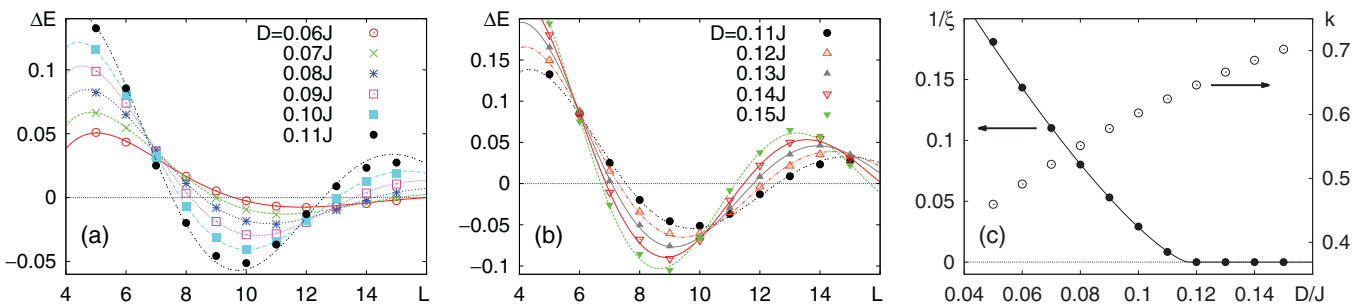
FIG. 5. (Color online) The splitting of the ground-state doublet as a function of the system length L for (a) D < D_c = 0.115J and (b) for D > D_c . (c) The dependence of the inverse tunneling length 1/\xi and the wave number k in the scaling form (13) on the DM coupling (strength) D .
