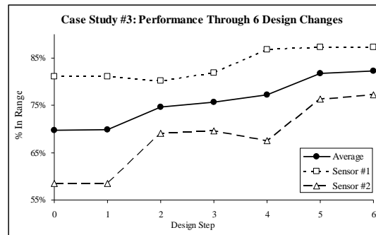
Figure 10 Case Study #3 performance improvement over 6 steps (12% total for the average of both sensor planes)
