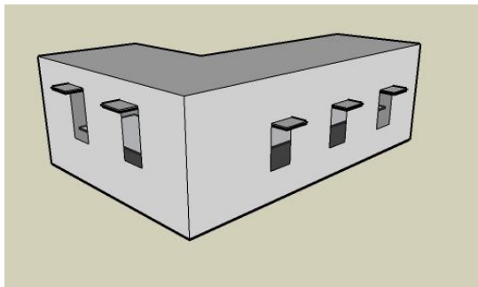
Figure 6 Case Study #2 design after 6 steps (Goal: 200 lx minimum, 800 lx maximum)
