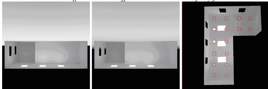
Figure 1 Sample renderings of a test scene using Radiance (left image) and LSV (middle image) at noon on March 21. The right image shows the same scene with the 16 area sensors distributed across the working plane.
