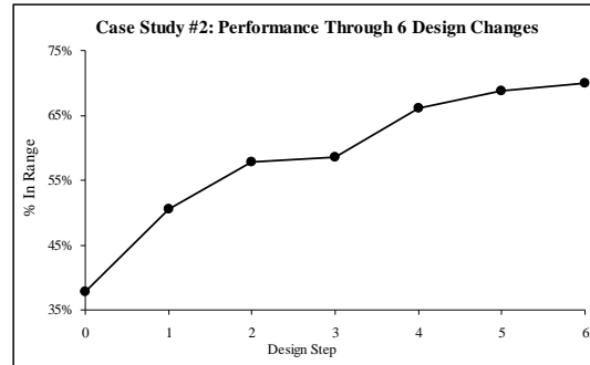
Figure 7 Case Study #2 performance improvement over 6 steps (32% total)
