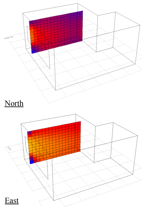
Figure 5: DA in a Vertical Plane at the Patient’s Head (“+”), see Figure 3 above, GF=30%, Max Illumin (100%) = 190 lux E, 180 lux N, (0600-1800h). Yellow/Light = 100%, Blue/Dark = 50%. Location: Boston, USA.
