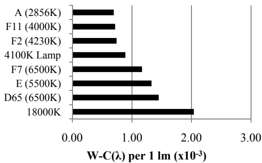
Figure 1: Circadian-Weighting of Illuminants
