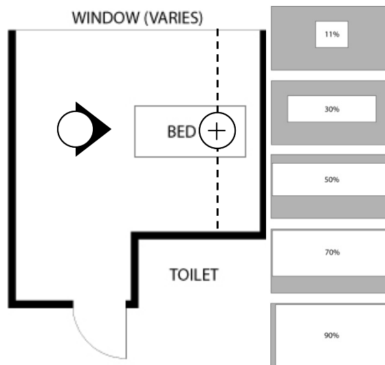
Figure 3. L: Hospital patient room configuration. Test point is noted by “+” and vertical illuminance test plane by a black dashed line as viewed from the elevation marker at the foot of the bed. R: test window configurations by glazing factor (%).
