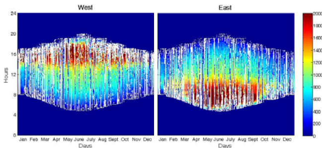
Figure 6: Temporal Maps of West (L) and East (R) Facing Patient Room, GF=90%, Max Illumin = 2000 lux, Min Illumin. = 0 lux. No Shading Device or Blinds Specified. Vertical axis: time (0 h, bottom to 24 h, top). Horizontal axis: day/month of year (Jan, L. to Dec, R.). Location: Boston, USA.
