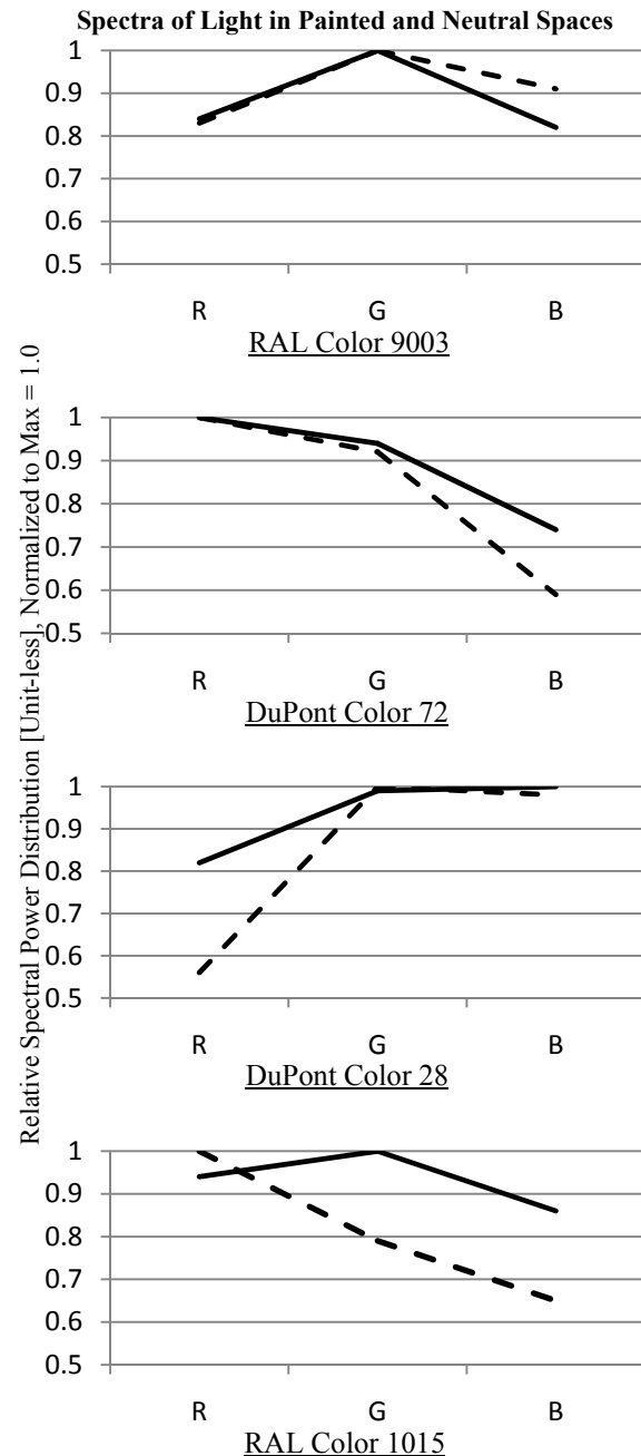
Figure 7: Radiometric RGB for Hypothetical (Dashed) and Simulated Spectra (Solid), Normalized to 1.0, D75 Sky
