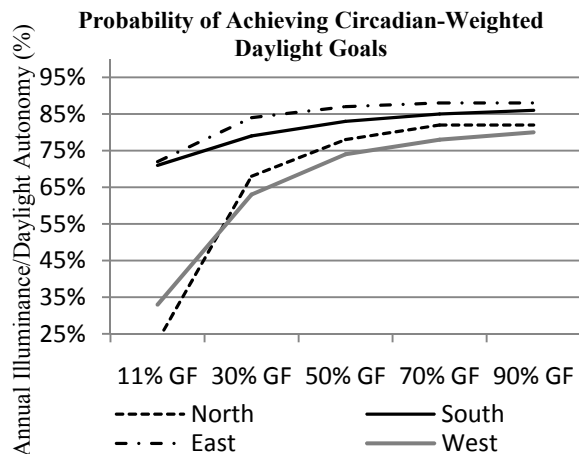
Figure 4: DA (%) at Test Point (190 lux or 180 lux (north), 06:00-18:00h) by Glazing Fraction (%) for North, South, East, and West Facing Hospital Rooms in Boston, USA.
