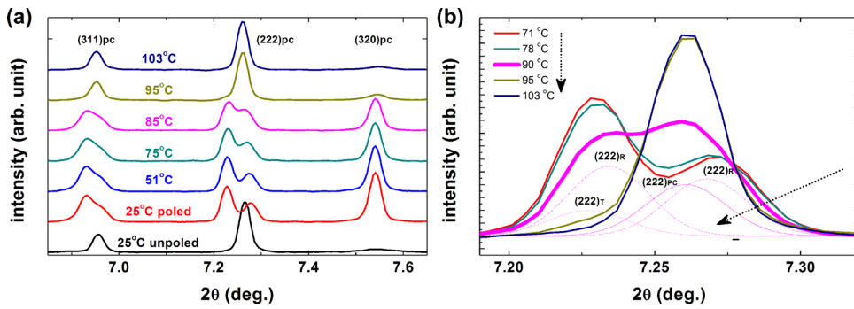
FIG. 3. (a) Three reflections in the XRD patterns for selected temperatures ( \lambda = 0.0143 nm) with the scattering vector, q , parallel to E , and (b) expanded view of \{222\}_{pc} for selected temperatures with the deconvoluted peak components of the \{222\}_{pc} at 90^\circ\text{C} . The position of each component was estimated by Rietveld analysis using FULLPROF, 28 and the deconvolution was done using Gaussian profiles.
