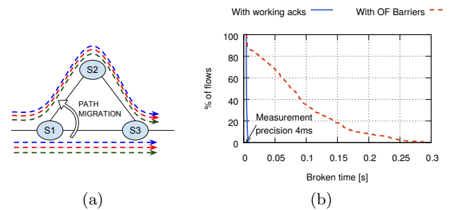
Figure 2: Consistent network update using a hardware switch. Despite theoretical guarantees, for most flows switch S1 gets updated before S2 and the network drops packets for up to 290 ms.
