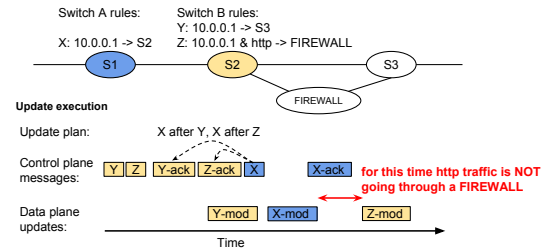
Figure 1: If switch B does not report data plane updates correctly, the theoretically safe update that adds rules for trusted and untrusted traffic from the same host turns into a transient security hole.
